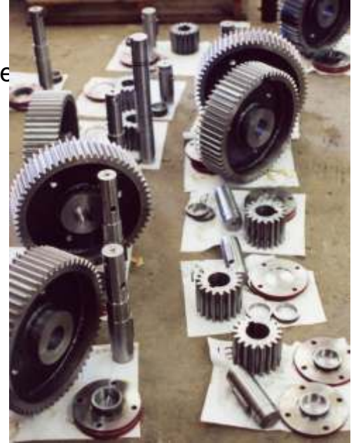
Precision made parts for a gear box. Everything from the gears, shafts, spacers, and even the main weldment are machined and fabricated at Industrial Wood
